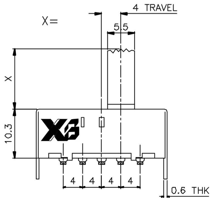
SLIDE SWITCH 1P3T
