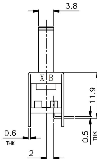
SLIDE SWITCH 1P4T
