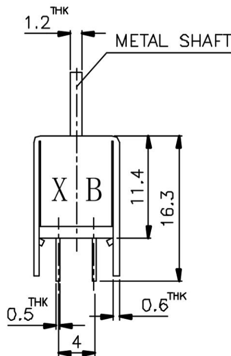
SLIDE SWITCH 2P3T
