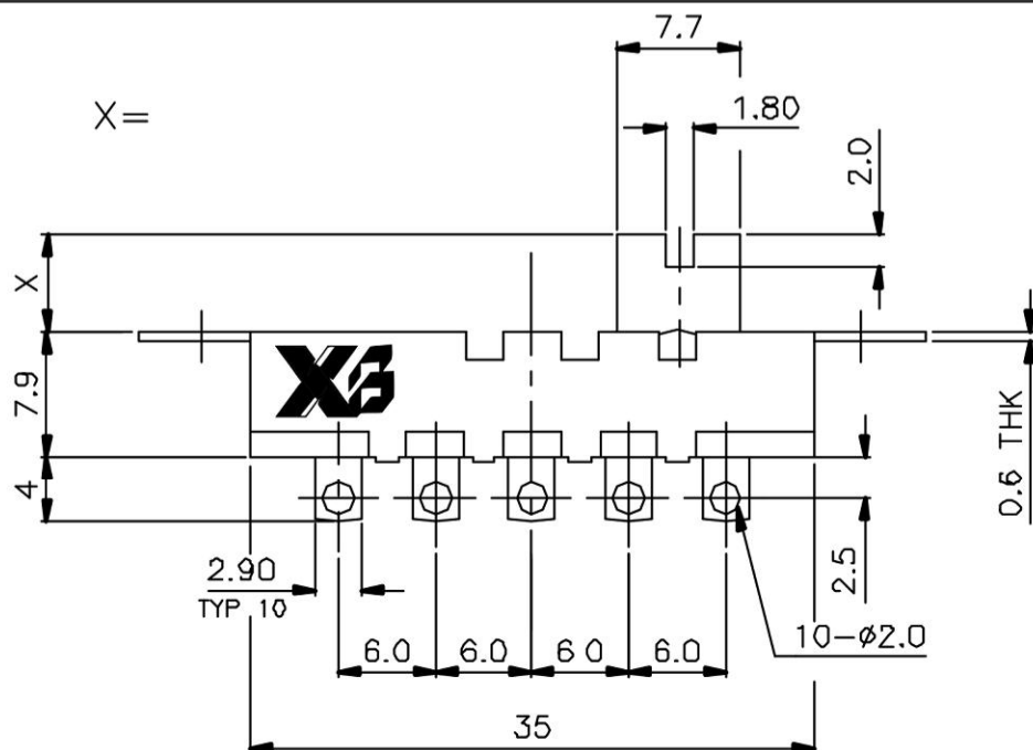
SLIDE SWITCH 2P4T
