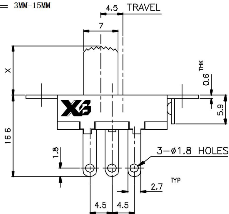
SLIDE SWITCH 1P2T
