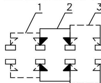
NON-SHORTING SCHEMATIC
