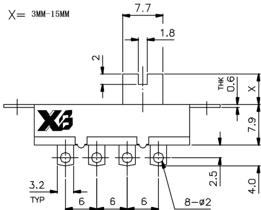
SLIDE SWITCH 2P3T
