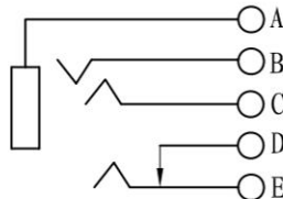
ST-166A SCHEMATIC
