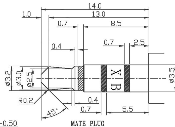
SCHEMATIC
