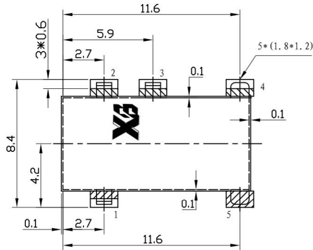
P. C. B LAYOUT
