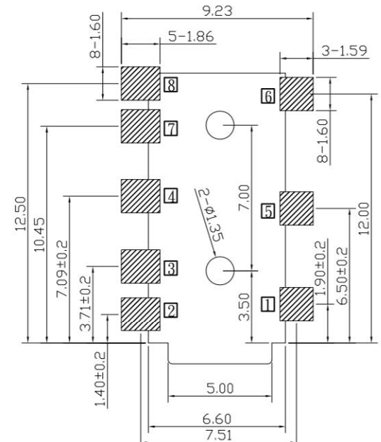
RECOMMENDED PCB LAYOUT(TOP VIEW)
