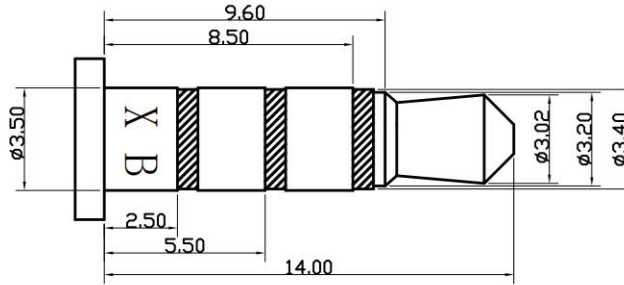
Ø3.50mm 4 POLE PLUG DETAIL DRAWING (1:1)
