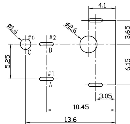
PCB LAYOUT
