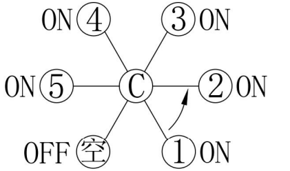
ON-ON-ON-ON-ON-OFF 电气原理图
