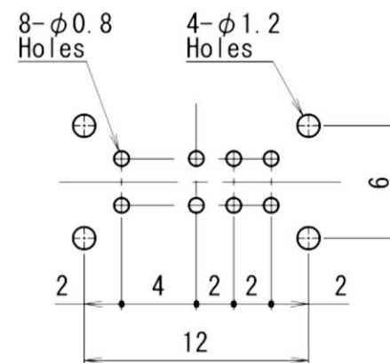
PC board mounting hole dimension (TOP VIEW)
