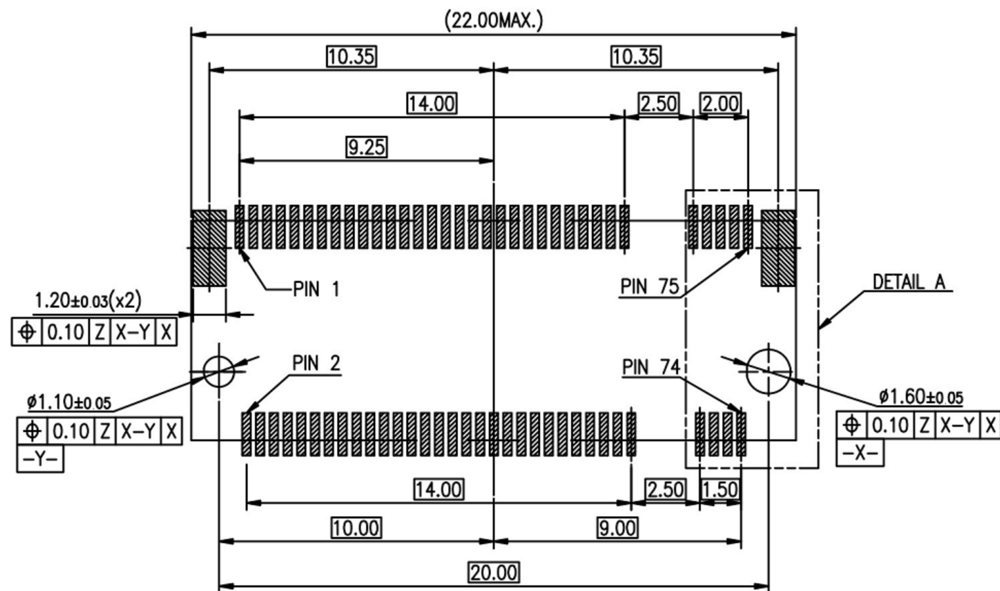
RECOMMEND PCB LAYOUT(TOP VIEW) (DEFAULT TOLERANCE:±0.05mm)
