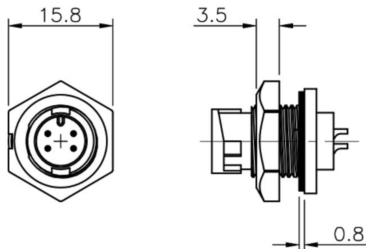
Assembly View
