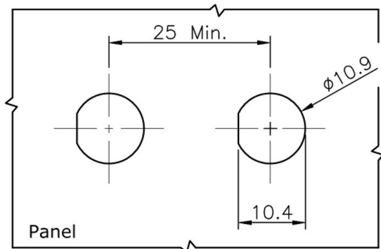
Recommend Panel Cut
