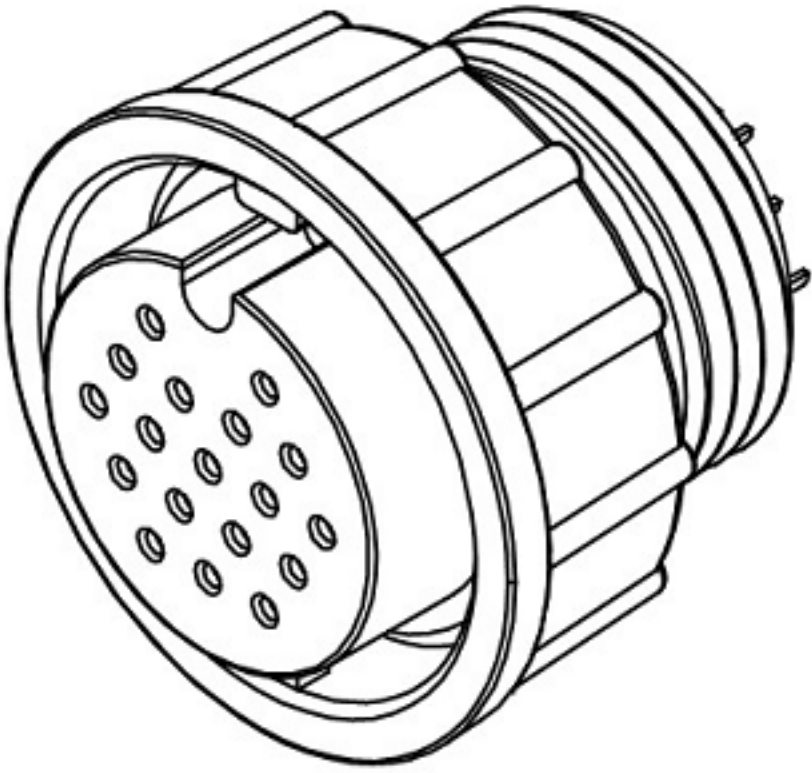
Drawing Number: 227D-MFF0 Description: D size connector, overmolding cable lock bayonet, female socket female pin, solder bucket
