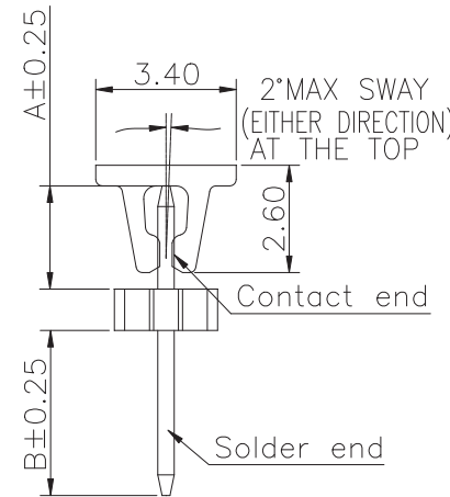
GPEA108 No Stand-off
