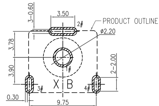
RECOMMENDED PCB LAYOUT TOP VIEW TOLERANCE: \pm 0.05
