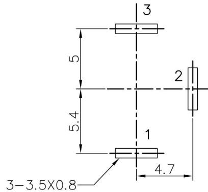
PCB Holes diagram Top View
