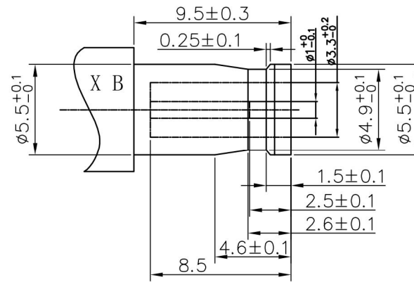
Matching Plug
