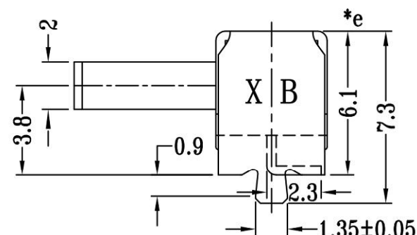
SIDE KNOB SLIDE SWITCH 1P5T
