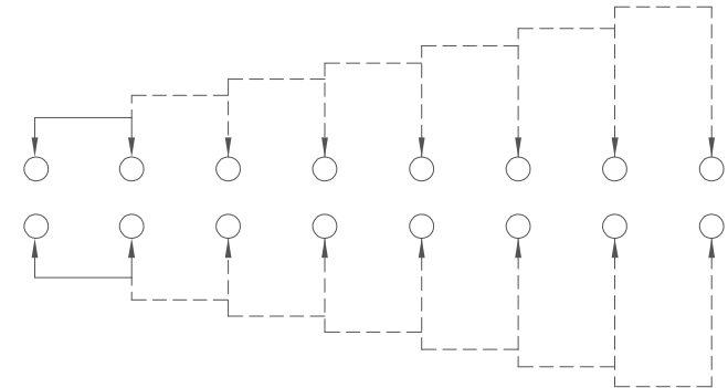
SCHEMATIC (NON-SHORTING)
