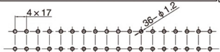
PCB LAYOUT
