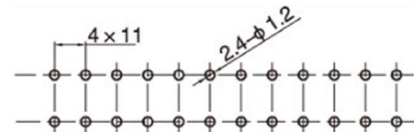
PCB LAYOUT
