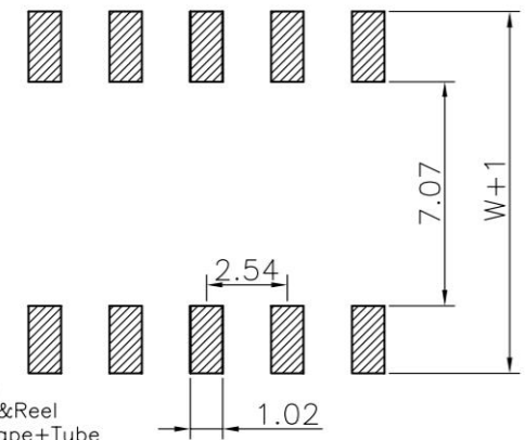
Recommended P.C.Board Layout (Tolerance:±0.05)
