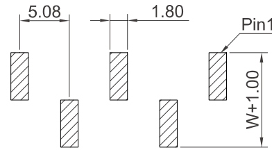
Recommended P.C.Board Layout (Tolerance:±0.05)
