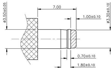
(3.50mm DC PLUG DETAIL DRAWING)
