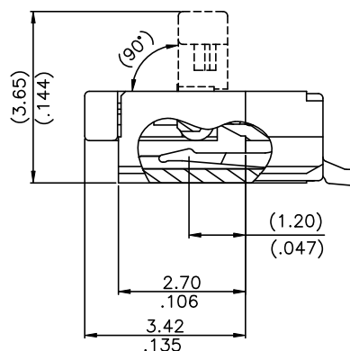
COVER OPEN STATE
