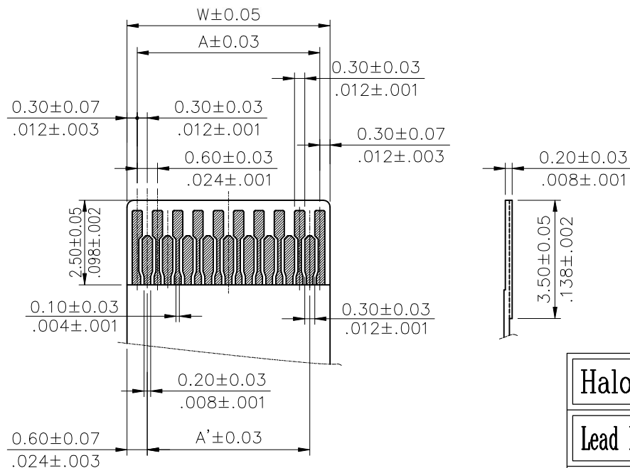
Accommodated FPC
