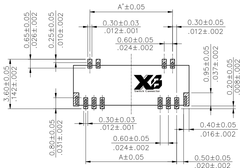
Recommended PCB Layout(Top View) Recommended metal mask pattern(thickness 0.1mm)
