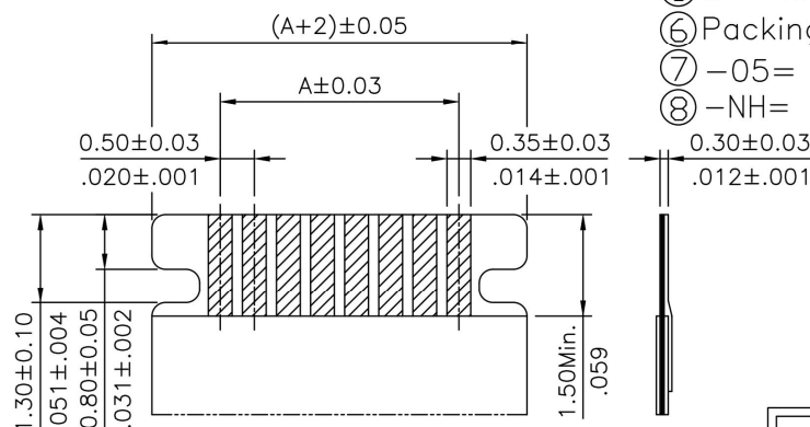
Accommodated FFC/FPC
