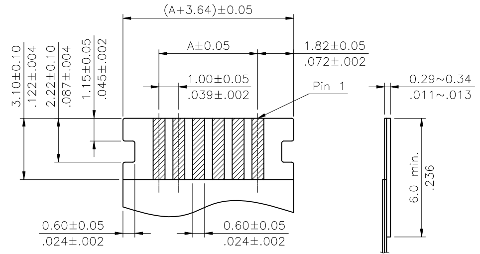
Accommodated FFC/FPC
