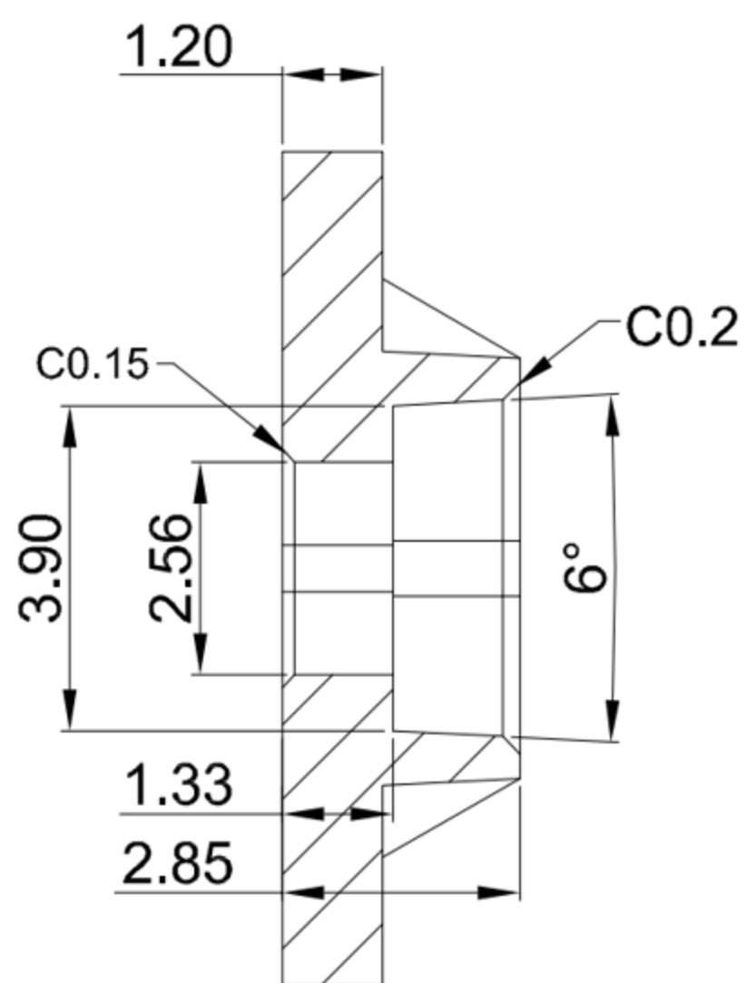
SECTION B-B
