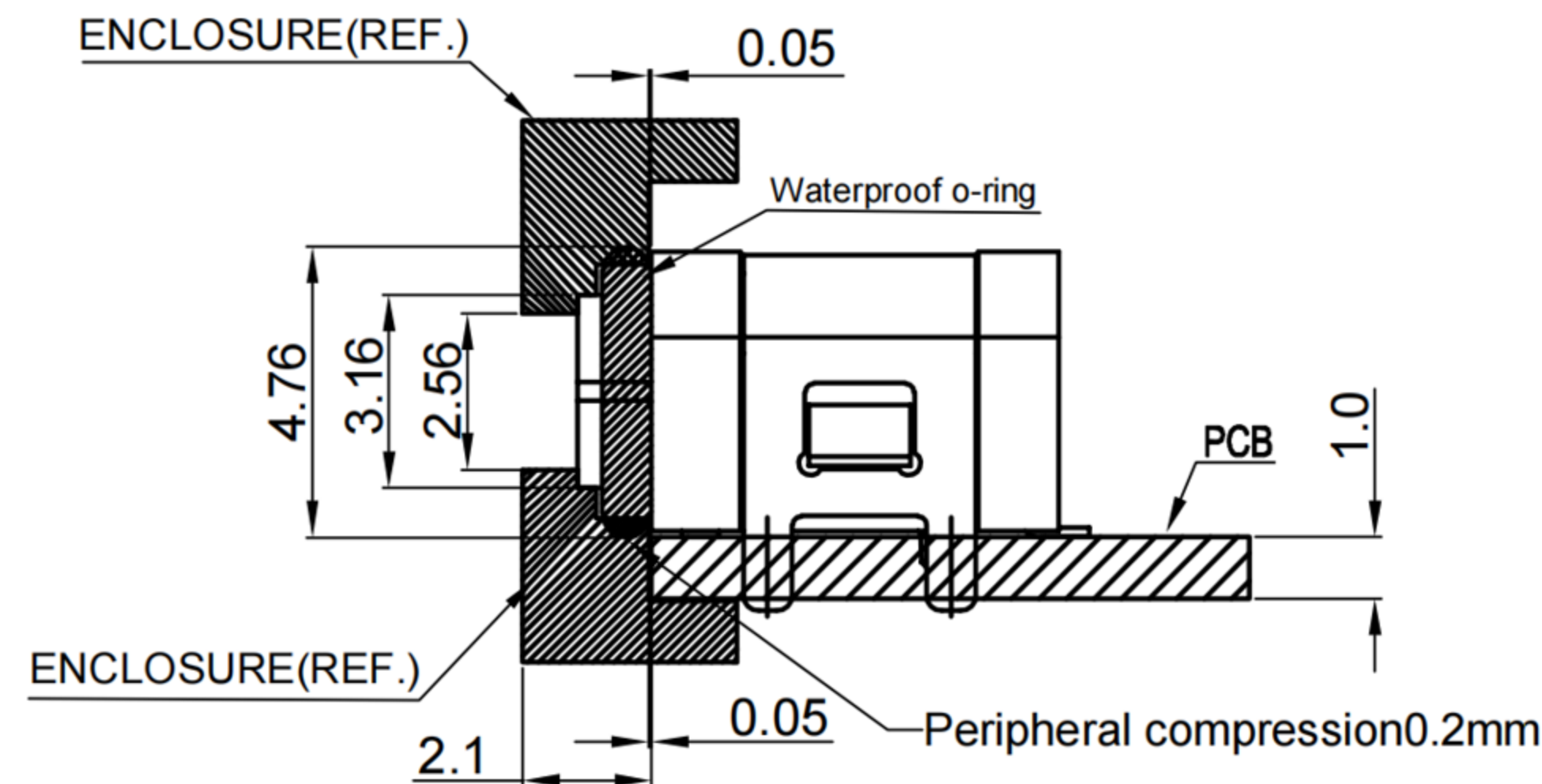
RECOMMENDED ASSEMBLY DRAWING
