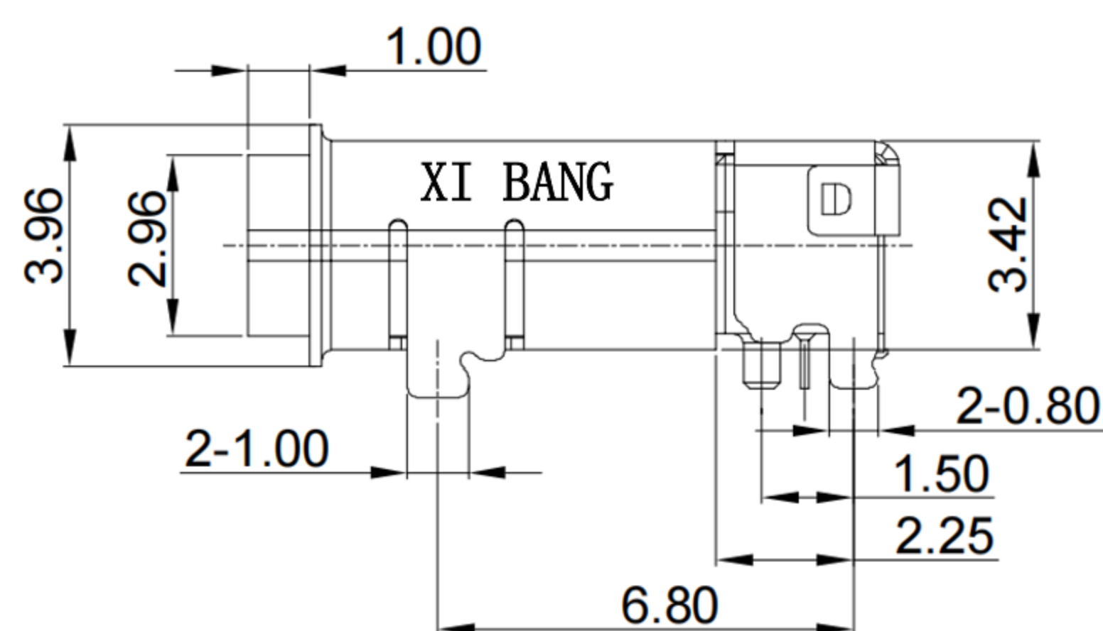
SECTION B-B
