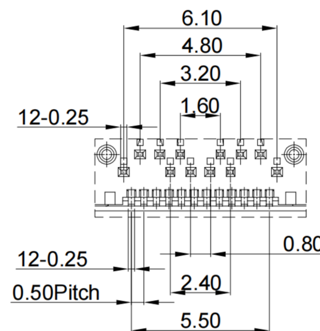
DETAIL A
