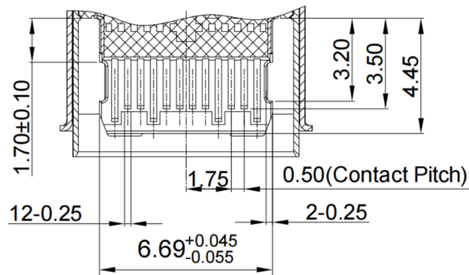
SECTION B-B
