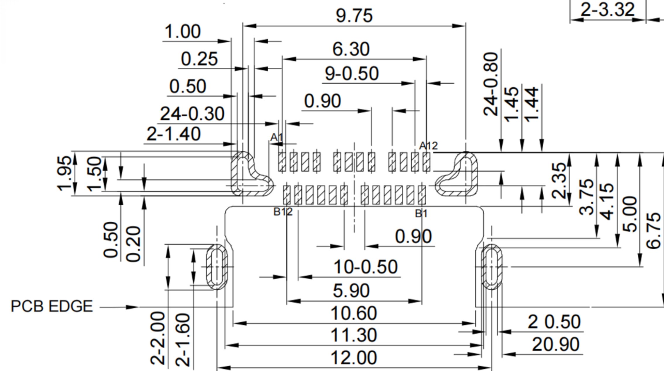
RECOMMENDED PCB LAYOUT TOLERANCE: ±0.05
