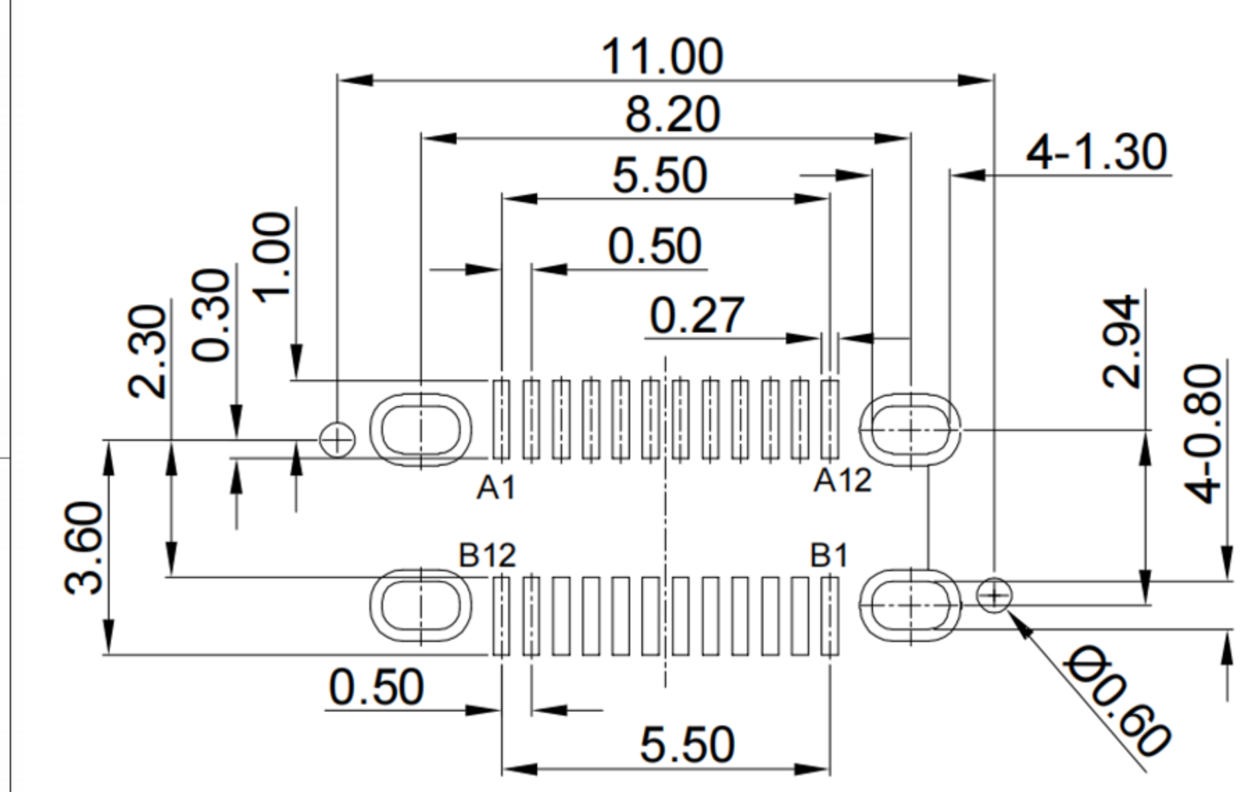
RECOMMENDED PCB LAYOUT TOLERANCE ±0.05mm
