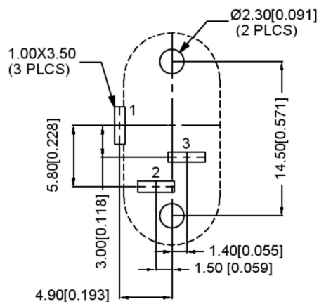
PCB LAYOUT FRONT VIEW
